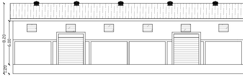
ELEVATION SCALE 1:100
