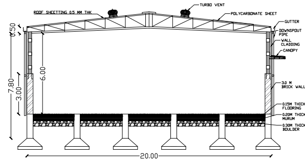
SECTION X-X' SCALE 1:100
